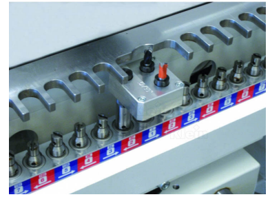
DRILLING JIG FOR MAKING HOLES FOR HINGE INSERTING
