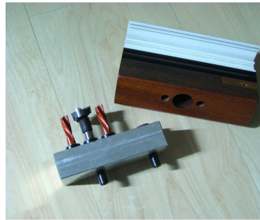
DRILLING OF WOOD AND PVC WINDOW FRAME TO FIT CREMONE BOLT
