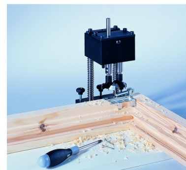
SPECIAL DEVICES FOR ANGULAR HINGES INSERTING
