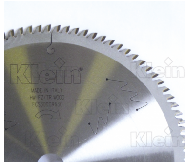
HW TRIMMING AND SIZING SAW BLADES
