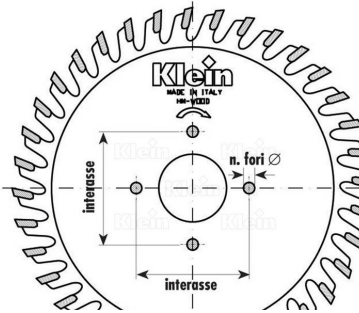
SAFETY PIN HOLES FOR SAWBLADES
