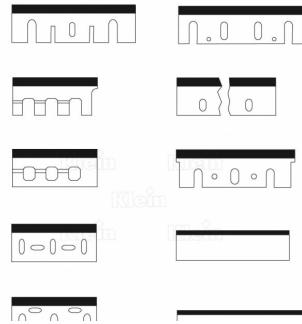
KNIVES FOR PORTABLE PLANERS
