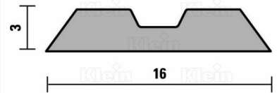
TURNBLADES "CENTROLOCK"
