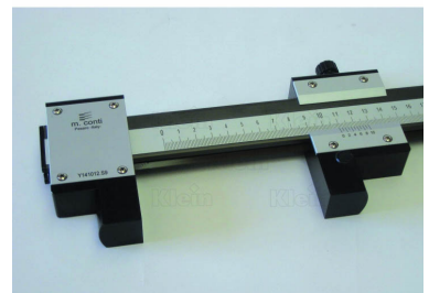
GAUGE FOR INSIDE/OUTSIDE MEASURING
