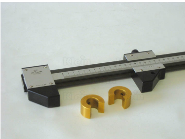
GAUGE FOR DIAGONAL AND OUT OF SQUARE MEASUREMENTS
