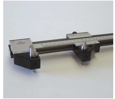
GAUGE FOR LINEAR MEASUREMENTS, DISTANCE FROM THE CENTRES OF THE HOLE TO THE EDGE OF THE PANEL
