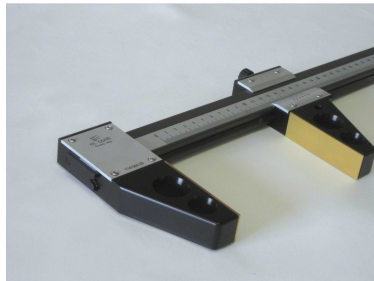
GAUGE FOR LINEAR MEASUREMENTS, WITH LONG JAWS AND STEEL PLATES
