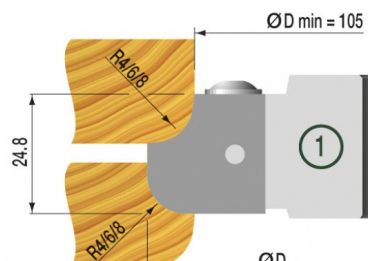
HW TOOLING SET FOR CONCAVE AND CONVEX QUARTER ROUNDS
